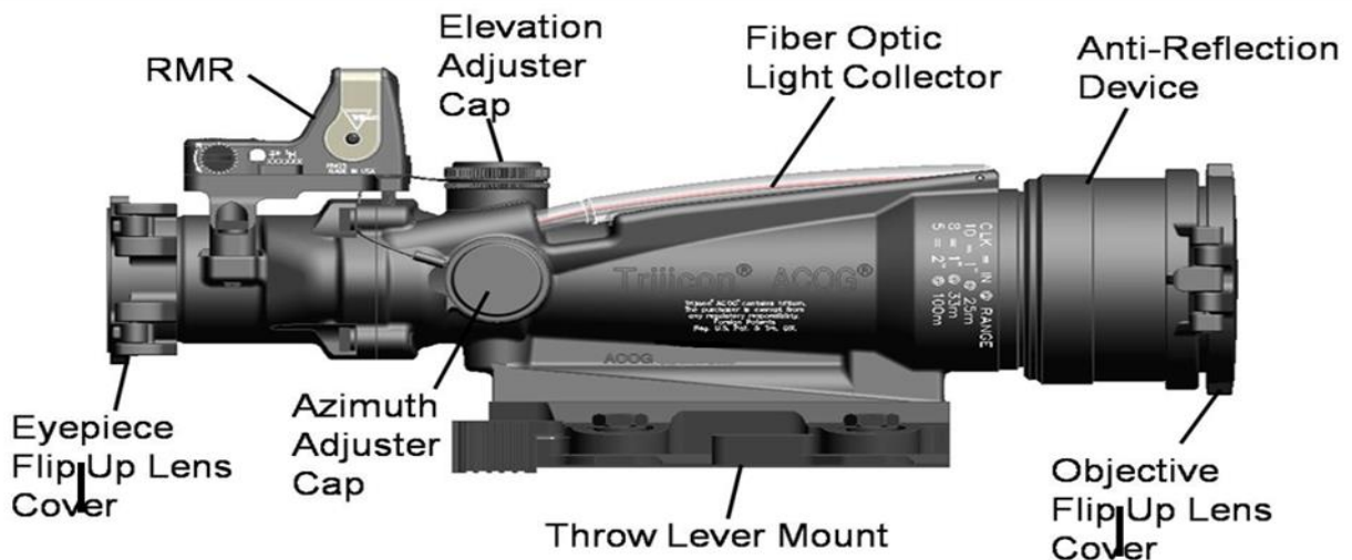
TA11 Squad Day Optic (SDO)
