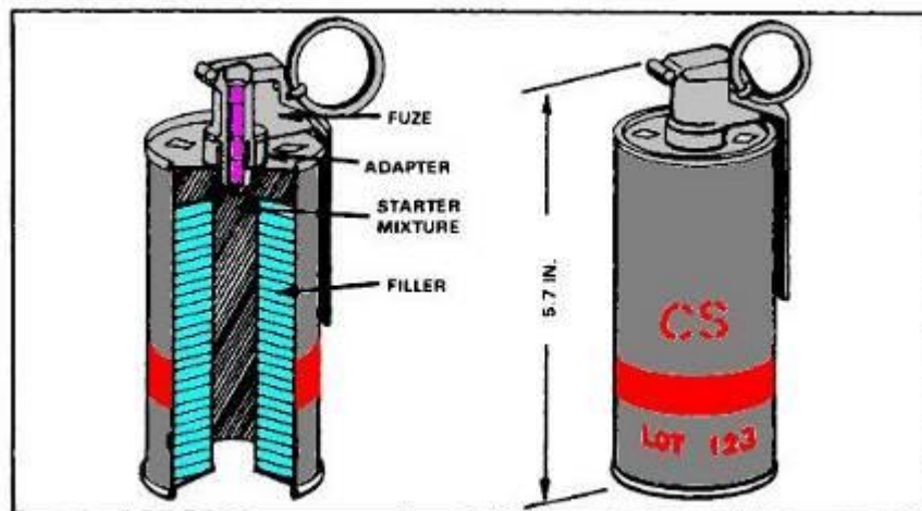
ABC-M7A2 and ABC-M7A3 riot control grenades.
