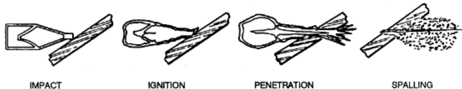
Effects of LAW Warhead
