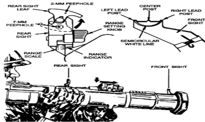
Sight Location and Resemblance to M16 Series Rifle Sights
