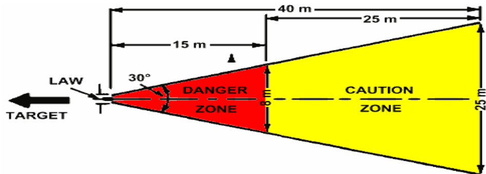
M72 LAW Back Blast
